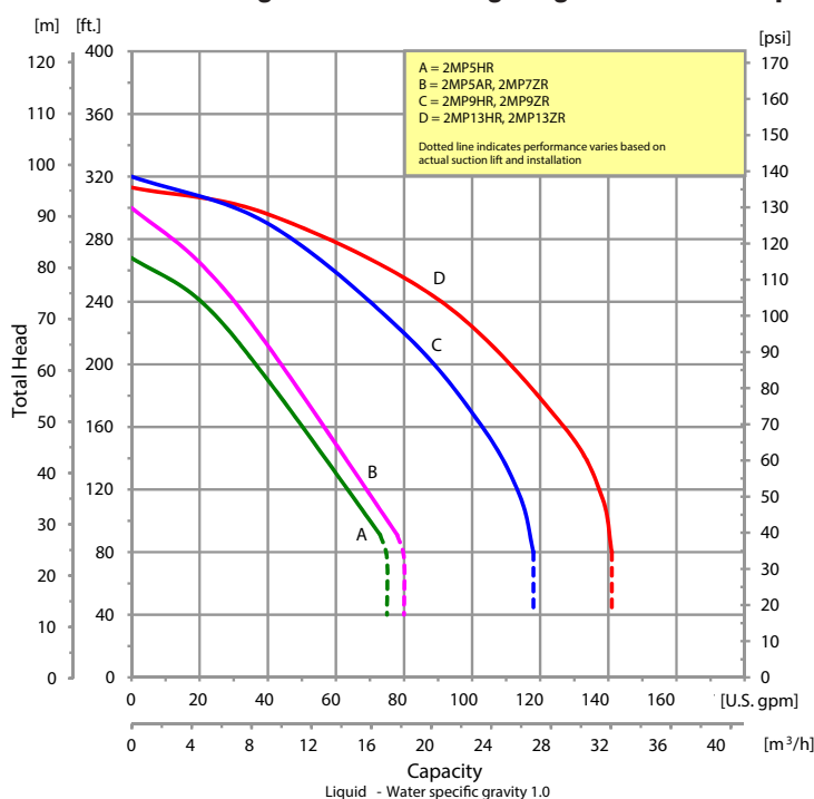
Performance of Engine-Driven 2-Stage High Pressure Pumps
