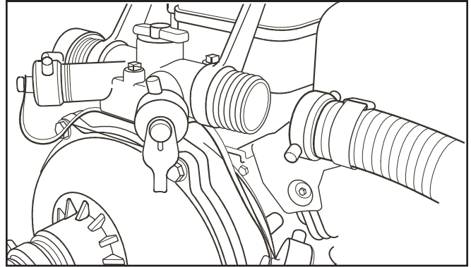
Figure 4 - Attach Discharge Hose to Pump
