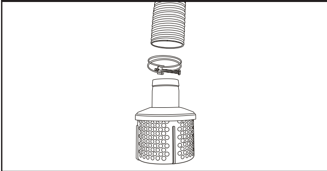
Figure 3 - Attach Suction Hose to Strainer Basket
